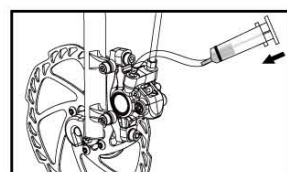
f-6. Fill the reservoir with oil by pushing the syringe
